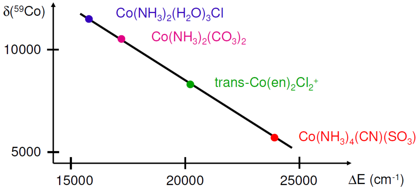
Relationship between \delta(^{59}\text{Co}) and the excitation energy of lowest d \rightarrow d^* electronic transition
